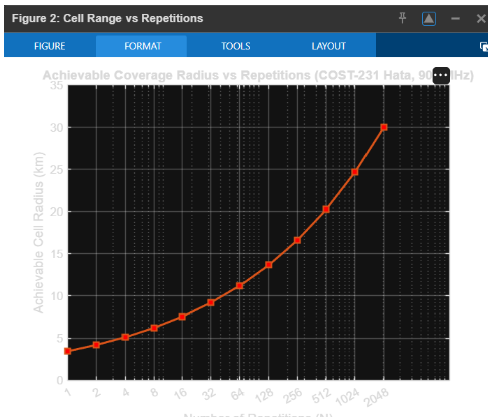
Figure 3: Achievable cell radius versus number of repetitions (COST-231 Hata, 900 MHz)
