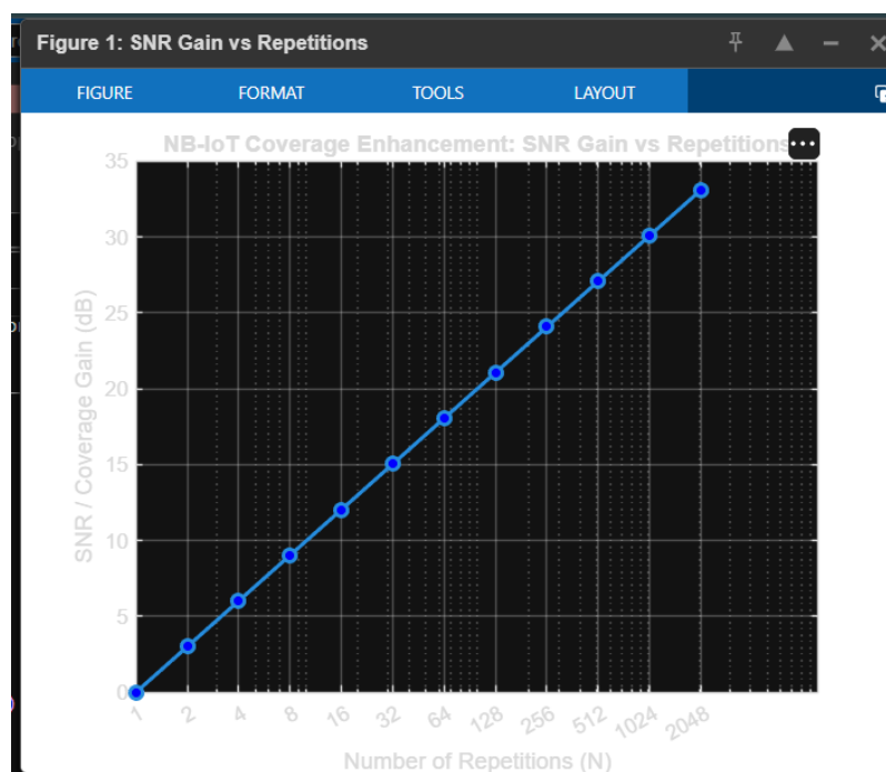
Figure 2: SNR / coverage gain versus number of repetitions
